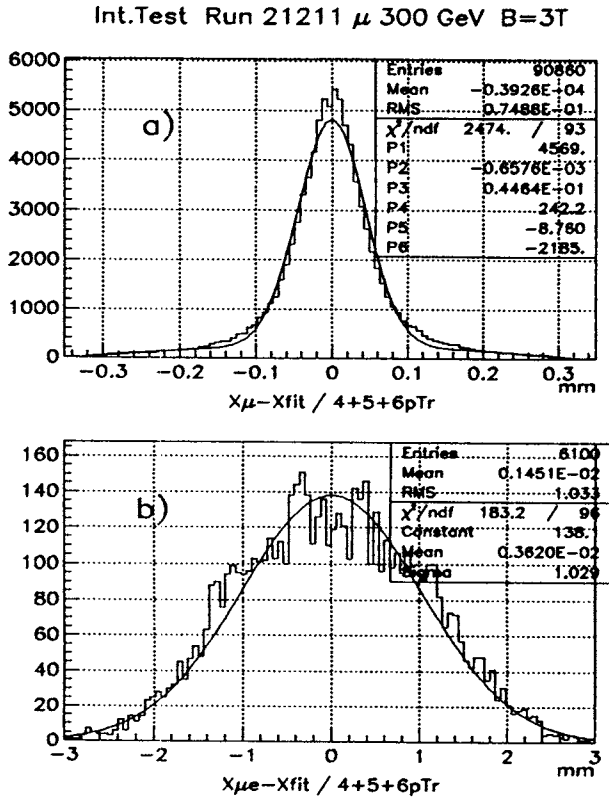
Fig. 5. The residuals (x_i - x_i^{fit}) : a) — for «good» \mu tracks (fitting with Gaussian + parabola), b) — for (\mu + e) tracks (fitting with Gaussian)
