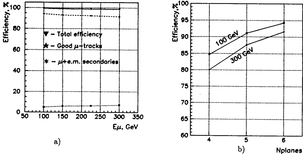
Fig. 6 a) The efficiency of muon-track reconstruction versus the energy of muon beam. The dashed line is the efficiency of «good» \mu -tracks reconstruction, the dotted line — the efficiency of ( \mu + e.m.secondaries)-tracks reconstruction and the solid line — the sum of them. b) The muon-track reconstruction efficiency dependence on the number of layers in ME1/1 chamber
